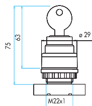
С ключом Key Operated
